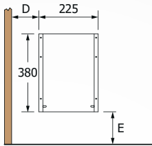
Wall Mounting Rack Installation
