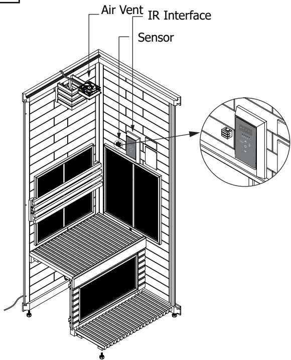
Fig. 3 Recommended location for the sensor
