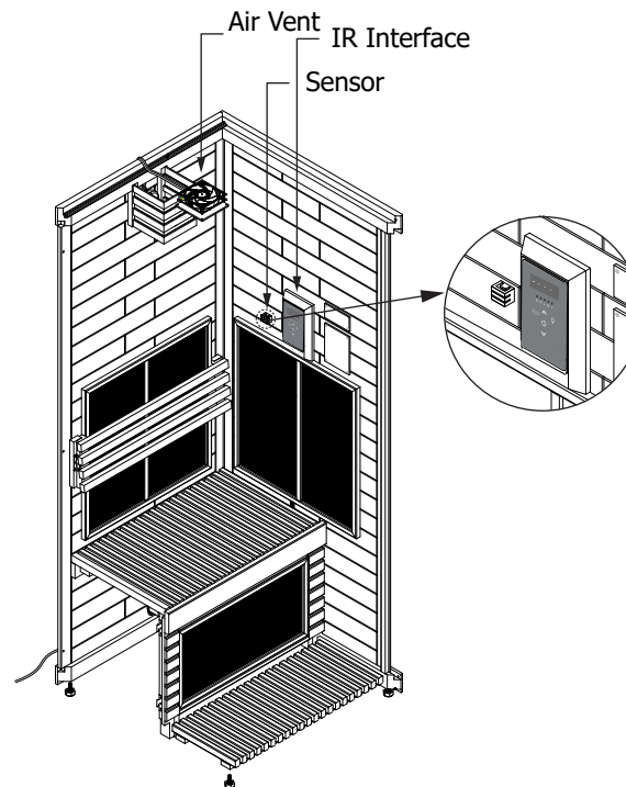
Fig. 4 Recommended location for the sensor
