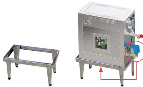
Installation Stand for STN-W code: STN-W-STAND
