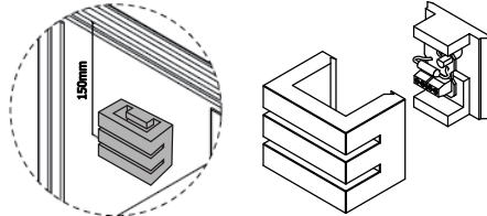
Temperature sensor with fuse on the wall
