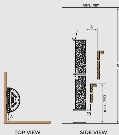
TOP VIEW SIDE VIEW Minimum Safety Distances
