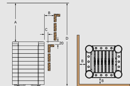
FRONT VIEW TOP VIEW Minimum Safety Distances
