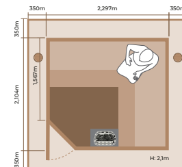
2125LLC INT. VOL.: 8.06 m 3 SCA 8.0 kW
