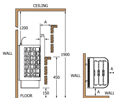
Side View Top View Minimum Safety Distances
