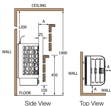
Minimum Safety Distances
