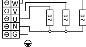
ARI3-60NS-WL 6,0 kW
