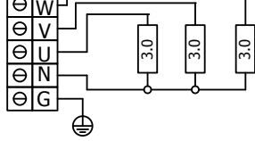
ARI3-90NS-WL 9,0 kW
