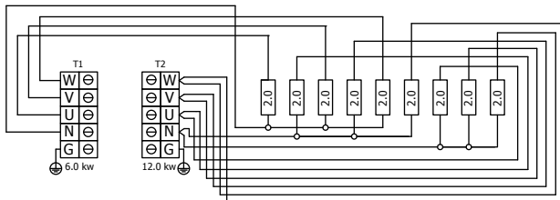
DRFT9-180NS 18,0 kW
