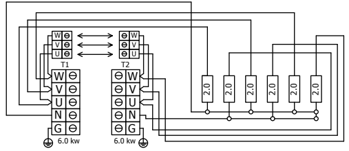
DRFT6-120NS 12,0 kW
